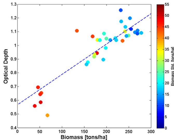
Fig. 10. Scatterplot of SMOS retrieved \tau_p vs. forest biomass measured in forest pixels of Peru and Columbia. Color codes indicate the standard deviation of measured biomass within SMOS pixels ( R^2 = 0.74 ) (Vittucci et al., 2016).
