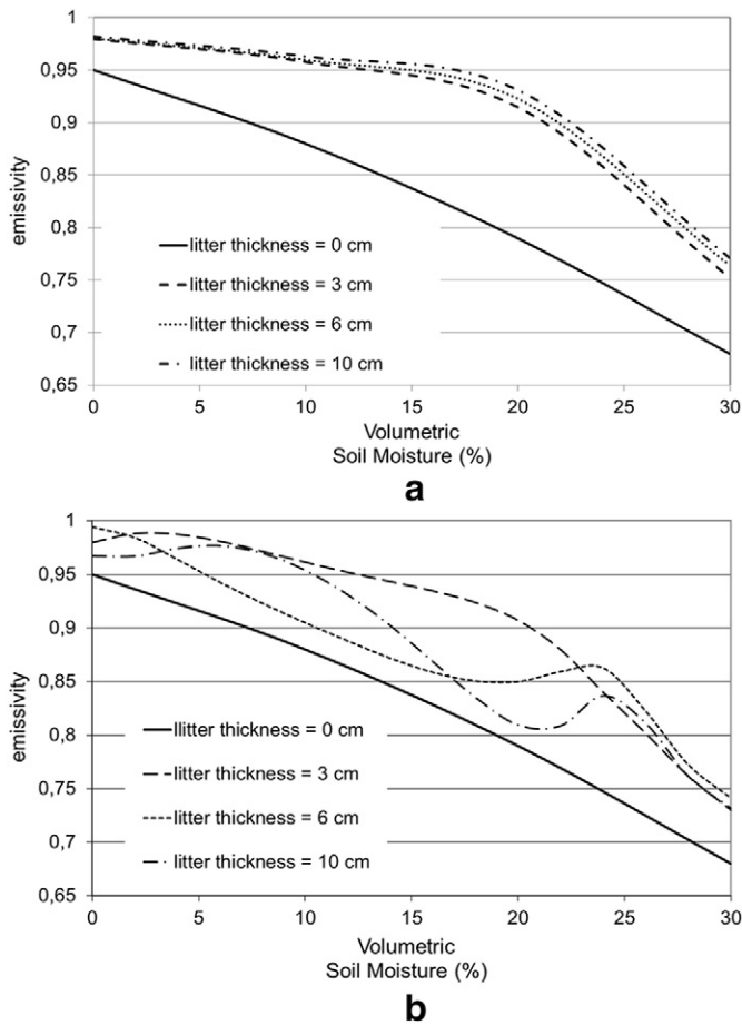
Fig. 11. Emissivity of a soil-litter system as a function of soil moisture for several values of the litter thickness (0, 3, 6 and 10 cm). Computations were made using an incoherent (a) and a coherent (b) model (Demontoux et al., 2008).
