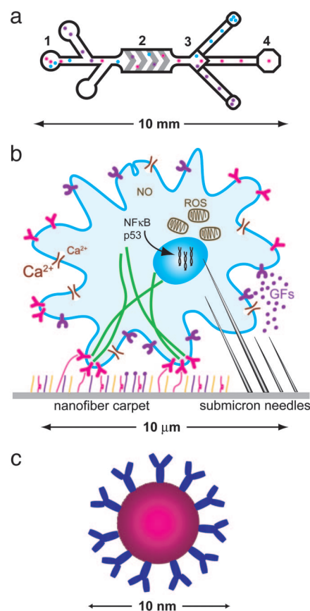
Fig. 1. Agents and length scales involved in designing a microchip-based nanoanalysis system to interface with living cells. ( a ) A typical microfluidic chip sequence illustrating circular sample/reagent introduction ports (label 1), reagent delivery to the main channel and subsequent mixing chamber (label 2), a sorting hub (label 3), and a cell isolation chamber (label 4). Colored dots represent living cells with different phenotypes that are treated, tagged, and/or sorted to stimulate or measure physiological activity profiles. ( b ) Cell isolation traps incorporate an array of submicrometer needles for stimulation or sensing in the cell nucleus (dark cyan), cytoplasm (light cyan), or extracellular space. A "nanofiber carpet" includes stretchable polymer chains to bind cell adhesion receptors and measure mechanical forces (magenta), filaments capped with growth factors (GFs, purple) that are either immobilized or released in soluble form, and nanowire electrodes (gold) to stimulate or measure electrical activity near the cell membrane. Data from these sensors comprise a "cell activity profile" consisting of mechanical events such as interactions within the cytoskeleton (green), production of reactive metabolites such as nitric oxide (NO) and reactive oxygen species (ROS), toxic gene regulatory responses such as activation of the transcription factors NF- \kappa B and p53, and transport of \text{Ca}^{2+} ions that contribute to signaling networks and transmembrane potential. ( c ) Schematic of a conjugated nanoprobe that could be targeted to protein complexes on or in the cell of interest using the submicrometer needles or nanofiber carpet.
