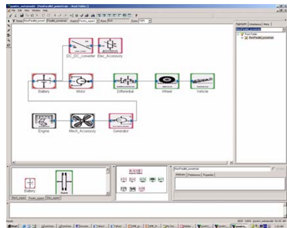
Figure 6. Series hybrid powertrain design in GME.
