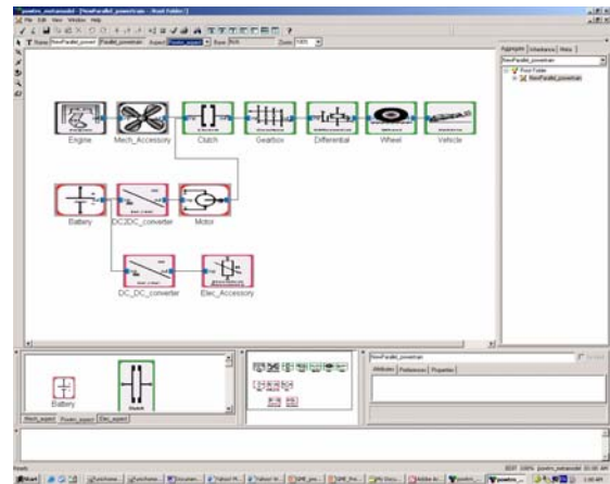
Figure 5. Parallel hybrid powertrain design in GME.
