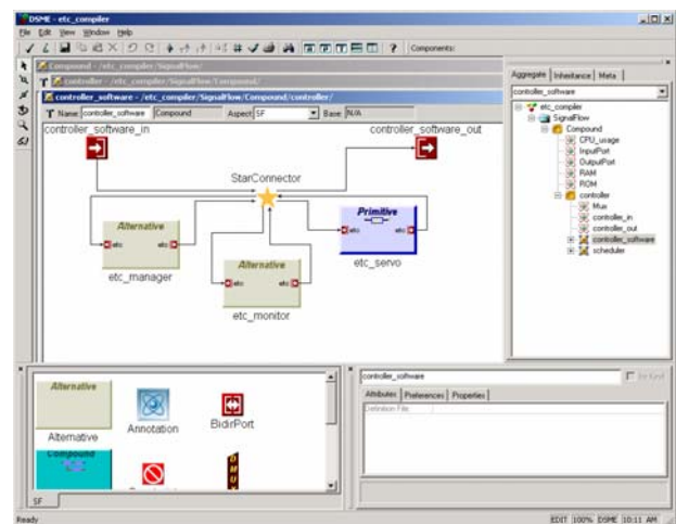
Figure 3. The Electronic Throttle Controller modeled in GME.
