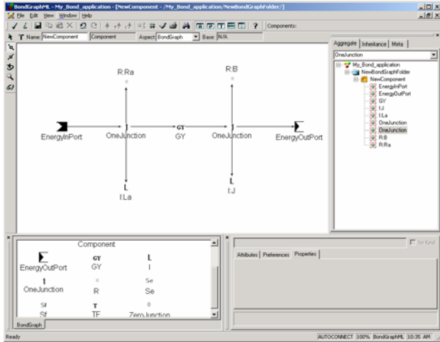
Figure 7. DC motor modeling using BG in GME.
