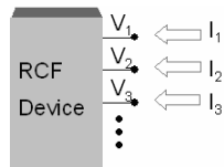
Figure 4. Physics-based Resistive Companion Form modeling technique.
