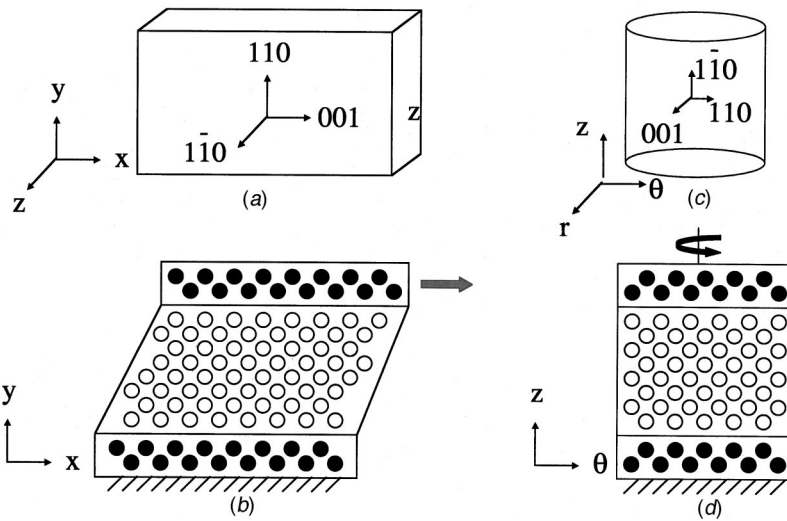
Fig. 5 Schematic of simulation block of atoms for (a) simple shear initial state, (b) simple shear at large strain, (c) torsion initial state, and (d) torsion at large strain in which the clear circles represent the active atoms and dark circles represent the boundary atoms
