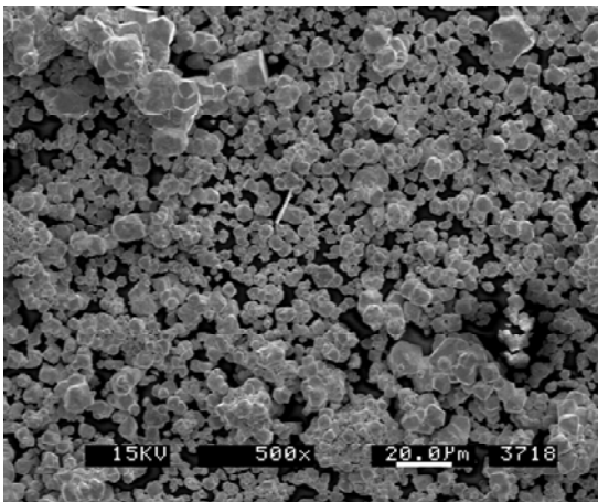
Figure 4 (a) - Particle morphology of the feedstock ( \phi = 60\% ) after mixing at 180 RPM for 120 min. in a torque rheometer.
